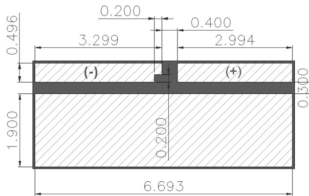
Bottom View (Pad)
